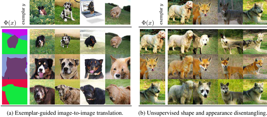
Figure 7: In (a), a segmentation representation \Phi(x) is translated under the guidance of the residual v = \tau^{-1}(\Theta(y)|\Phi(y)) obtained from exemplar y . In (b), \Phi is the same as \Theta , but applied after a spatial deformation of its input such that \tau learns to extract a shape representation into v , which then controls the target shape.
