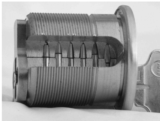
Figure 3: A lock with an incorrect key. Observe that while three of the pin stacks' cuts are at the shear line, two stacks have the cut too high and one stack has the cut too low.
