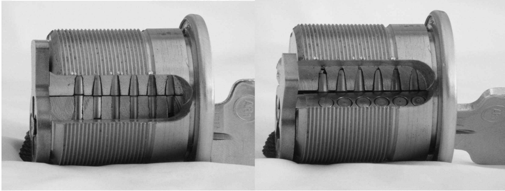
Figure 2: Pin tumbler lock with a correct key inserted. Left: The correct key lifts the pin stacks to align the cuts at the shear line. Right: With all of the cuts at the shear line, the plug can rotate freely within the shell. Here the plug has been turned slightly toward the camera, so that the tops of the pins in the plug are visible.
