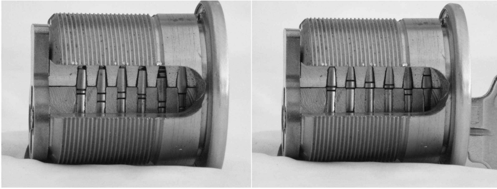
Figure 4: A master keyed pin tumbler lock. Left: Each of the six pin stacks has two cuts. Right: With the correct change key inserted, one of the cuts on each pin stack is aligned at the shear line. Observe that the other cut is sometimes above and sometimes below the shear line.
