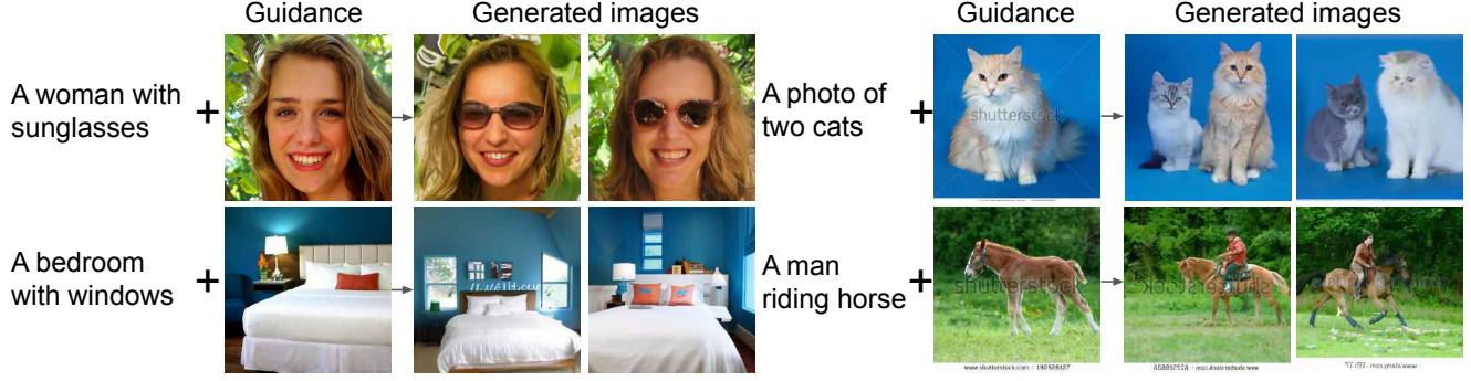
Figure 5. Image synthesis results with both image and language guidance. The image and language guidance provides complementary information, and our model generates images that matches both guidance.
