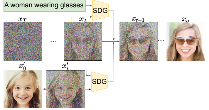
Figure 2. An overview of our method. We control the diffusion generation process by the Semantic Diffusion Guidance (SDG) with language and/or reference image. SDG is iteratively injected to each step of generation process.
