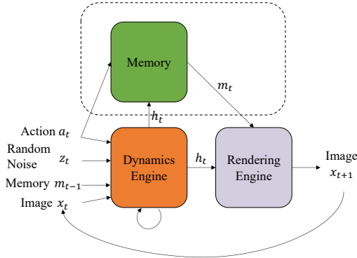
Figure 14: Overview of GameGAN: The dynamics engine takes a_t , z_t , and x_t as input to update the hidden state at time t . Optionally, it can write to and read from the external memory module (in the dashed box). Finally, the rendering engine is used to decode the output image x_{t+1} . The whole system is trained end-to-end. All modules are neural networks.
