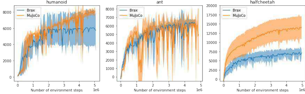
Figure 4: Qualitative comparisons of training curve trajectories in MuJoCo and Brax. (left) Training curves for MuJoCo-Humanoid-v2 and brax-humanoid, (middle) MuJoCo-Ant-v2 and brax-ant, and (right) MuJoCo-HalfCheetah-v2 and brax-halfcheetah. All environments were evaluated with the same standard implementation of SAC[28] with environments evaluated on CPU and learning on a 2x2 TPUv2—i.e., not Brax’s accelerator-optimized implementation. Solid lines indicate average performance, envelopes are variance over random seeds. See App. C for hyperparameters used. See Appendix E for a short discussion of the gap in performance for halfcheetah.
