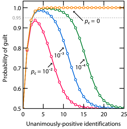
FIG. 2. Probability of guilt given varying numbers of unanimous line-up identifications, assuming a 50% prior probability of guilt and identification accuracies given by [17]. Of note is that for the case that we have plotted here where the witnesses are unanimous, with a failure rate p_c = 0.01 it is impossible to reach 95% certainty in the guilt of the suspect, no matter how many witnesses have been found.
