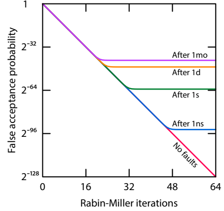
FIG. 5. The acceptance rate as a function of time in memory and the number of Rabin-Miller iterations under the single-error fault model described in this paper. An acceptance rate of 2^{-128} is normally chosen, however without error correction this cannot be achieved. The false-acceptance rate after k iterations is given by p_{fa}[k] = 4^{-k}(1 - p_f) + p_f , where p_f is the probability that a fault has occurred that causes a false acceptance 100% of the time. We estimate p_f to be equal to 10^{-19}T , where T is the length of time in seconds that the code has been in memory.
