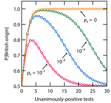
FIG. 1. Probability that the pot is of British origin given n numbers of tests, all coming back positive, for a variety of contamination rates p_c and a 30% error rate. In the case of the pot above, with p_c = 10^{-2} , we see a peak at n = 5 , after which the level of certainty falls back to 0.5 as it becomes more likely that the pot originates at a contaminating factory. When p_c = 0 , this is the standard Bayesian analysis where failure states are not considered. We see therefore that even small contamination rates can have a large effect on the global behaviour of the testing methodology.
