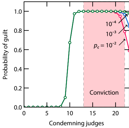
FIG. 3. Probability of guilt as a function of judges in agreement out of 23—the number used by the Sanhedrin for most capital crimes—for various contamination rates p_c . We assume as before that half of defendants are guilty, and use the estimated false-positive and false-negative rates of juries from [21, model (2)], 0.14 and 0.25 respectively. We arbitrarily assume that a ‘contaminated’ trial will result in the a positive vote 95% of the time. The panel of judges numbers 23, with conviction requiring a majority of two and at least one dissenting opinion [13, Sanhedrin]; the majority of two means that the agreement of at least 13 judges is required in order to to cast a sentence of death, to a maximum of 22 votes in order to satisfy the requirement of a dissenting opinion. These necessary conditions for a conviction by the Sanhedrin are shown as the pink region in the graph.
