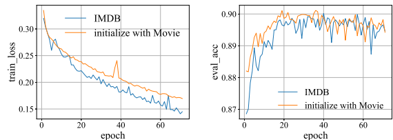
(a) IMDB training loss.
