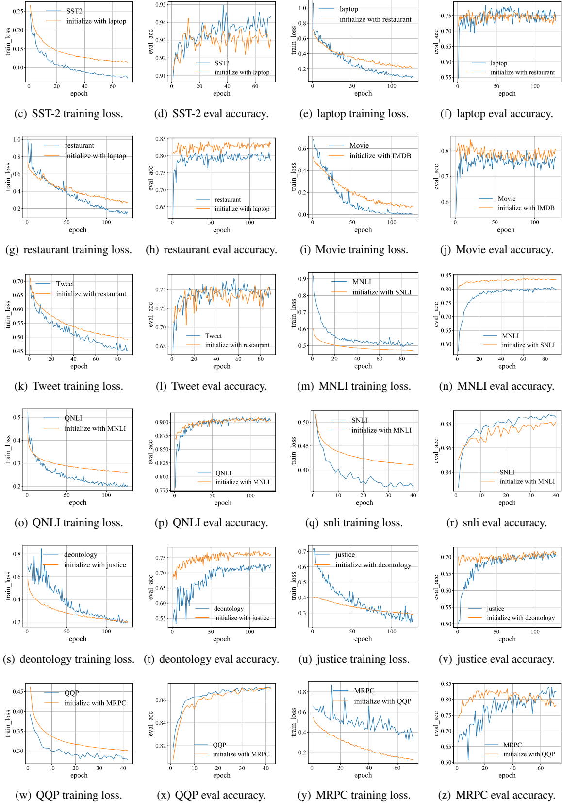
Figure 4: TPT TASK utilizes trained prompts from similar tasks as initialization for prompt tuning (—), which can mostly achieve better or comparable performance to vanilla PT (—) starting from random initialization and take fewer training steps to reach the comparable performance and convergence.
