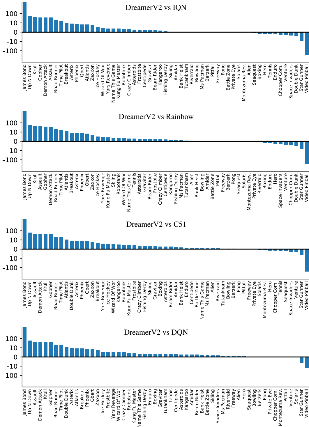
Figure E.1: Atari agent comparison. The bars show the difference in gamer normalized scores at 200M steps. DreamerV2 outperforms the four model-free algorithms IQN, Rainbow, C51, and DQN while learning behaviors purely by planning within a separately learned world model. DreamerV2 achieves higher or similar performance on all tasks besides Video Pinball, where we hypothesize that the reconstruction loss does not focus on the ball that makes up only one pixel on the screen.
