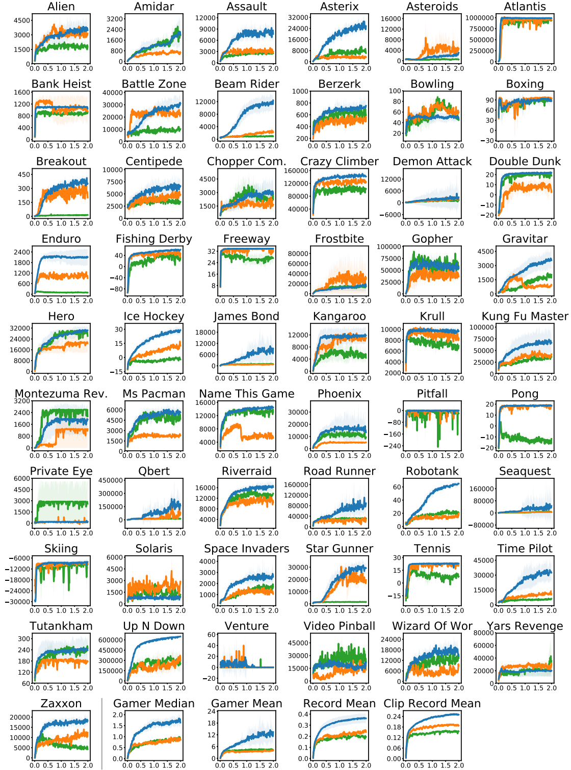
Figure G.1: Comparison of DreamerV2, Gaussian instead of categorical latent variables, and no KL balancing. The ablation experiments use a slightly earlier version of the agent. The curves show mean and standard deviation across two seeds. Categorical latent variables and KL balancing both substantially improve performance across many of the tasks. The importance of the two techniques is reflected in all four aggregated scores.
