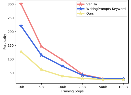
Figure 3: Convergence speed for different models.
