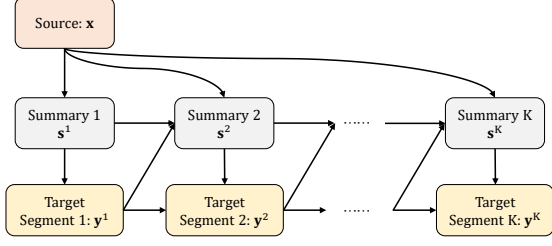
Figure 1: An overview of the proposed method. Given preceding tokens \mathbf{y}^{<i} , we first sequentially generate summaries \mathbf{s}^{j \sim k} for each snippet. Next we expand each summary \mathbf{s} to form the full text \mathbf{y}^{j \sim k} .
