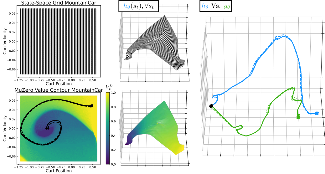
Figure 3. Left: Relation between true state space and latent state space on MountainCar. The top-left maps the true state space, indexed by vertical lines, into the latent space, retaining the vertical lines. The pattern indicates that the latent space gets curved, stretched and compressed. The bottom-left shows the same mapping, but this time indexes the states by their value estimate near convergence. We see that the latent embedding groups states that are dynamically close, which is visible in the grouping of states with similar values (in MountainCar, states that are dynamically close also have similar value, since there is only one start region and one sparse goal). Right: Latent embedding of a ground truth trace pushed through the encoder h (blue) and latent embedding of the same trace embedded at the first state and subsequently propagated at latent level through g . We clearly see that, although both traces should cover the same trace and cumulative reward, their latent trajectories diverge.
