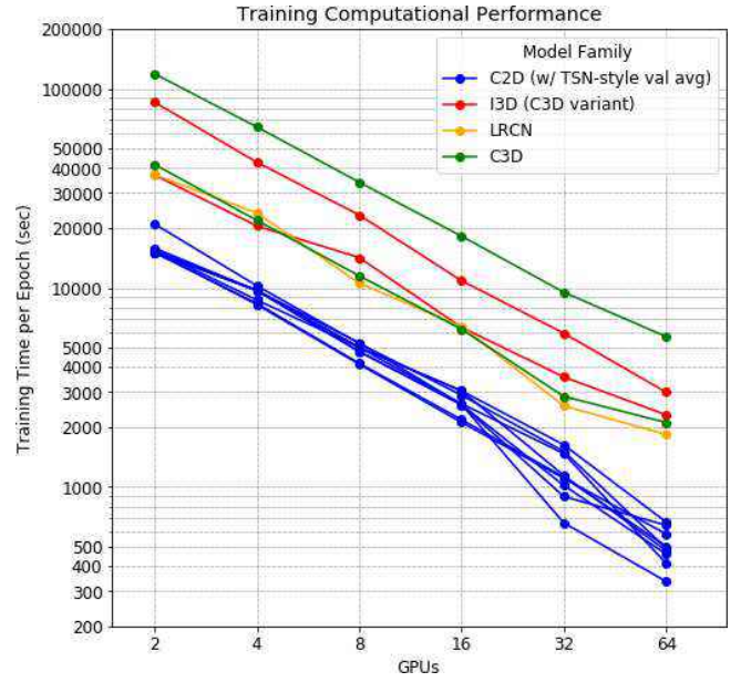
Fig. 4. Training Time per Epoch across training configurations of 1, 2, 4, 8, 16, and 32 nodes where each node as 2 Volta V100 GPUs.
