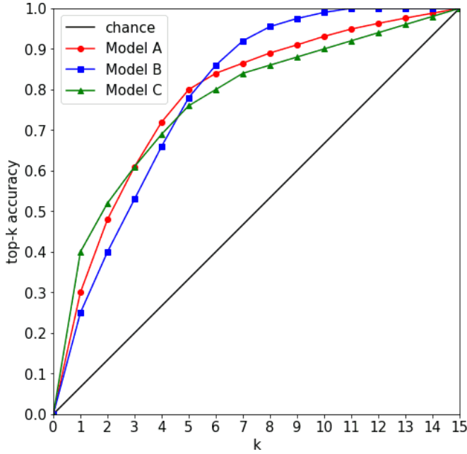
Fig. 2. Example p-ROC curve for a 15-class problem. Three model Top- k values are plotted (as well as a random chance line that represents an uninformed guesser).
