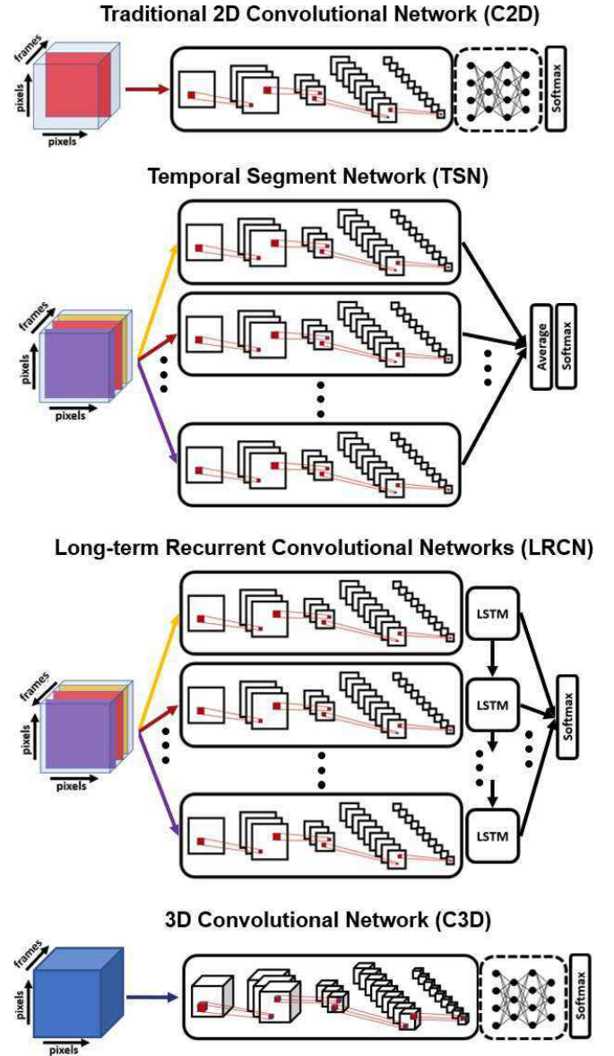
Fig. 1. Common video action recognition approaches. Note that these are simplified where icons for 2D-ConvNets, 3D-ConvNets, dense classification networks, LSTM modules, and averaging/softmax layers are used only as visual interpretation. Their actual design can vary significantly. Similarly, the majority of approaches have 2-stream variants for RGB+Optical Flow.
