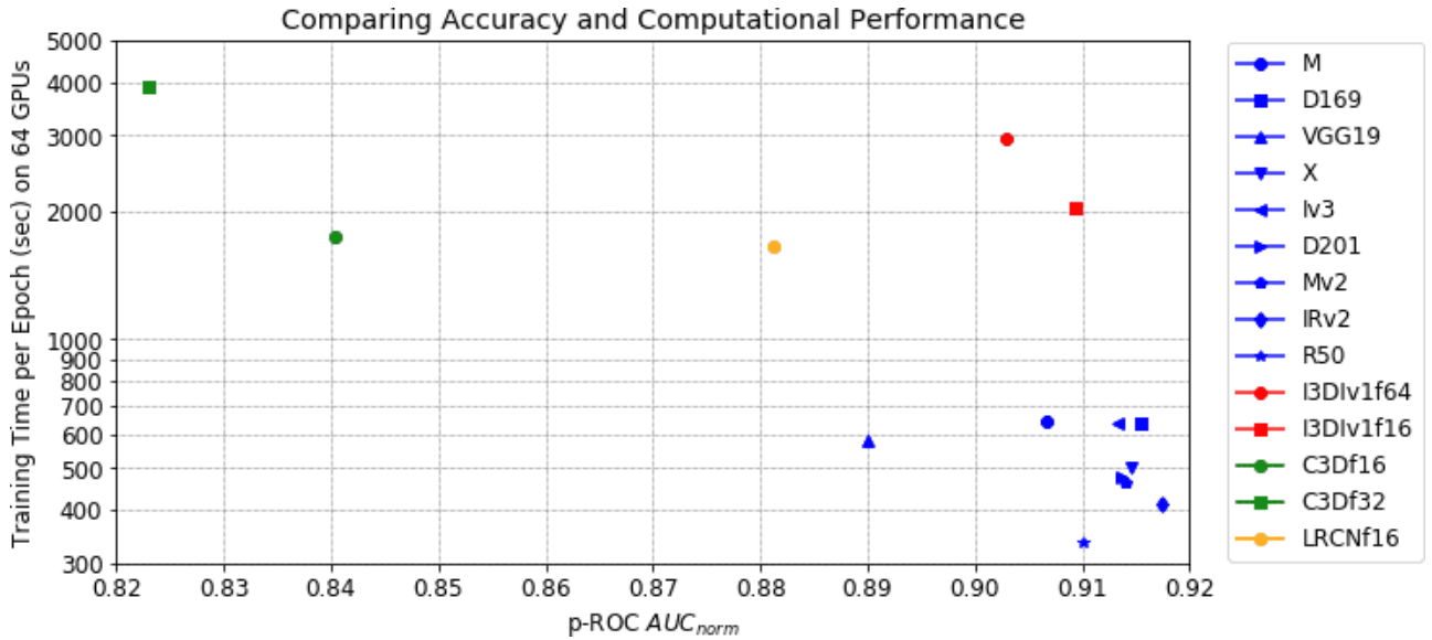
Fig. 5. A plot of training time per epoch (measured in seconds) against p-ROC \widehat{AUC} = AUC_{norm} to show accuracy and computational performance trade-offs. The best performing models are found in the lower-right corner.
