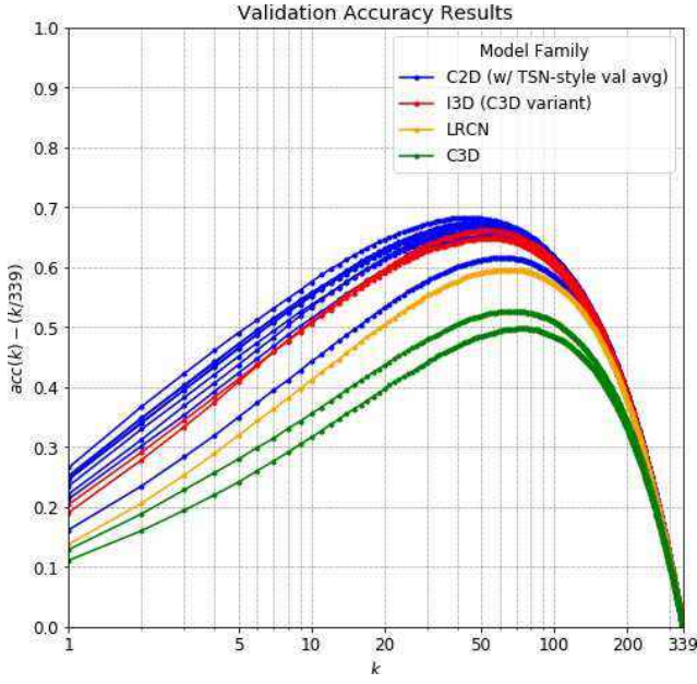
Fig. 3. p-ROC curve log-scaled with k/339 subtracted out for each value of k to more easily show the peak J -statistic
