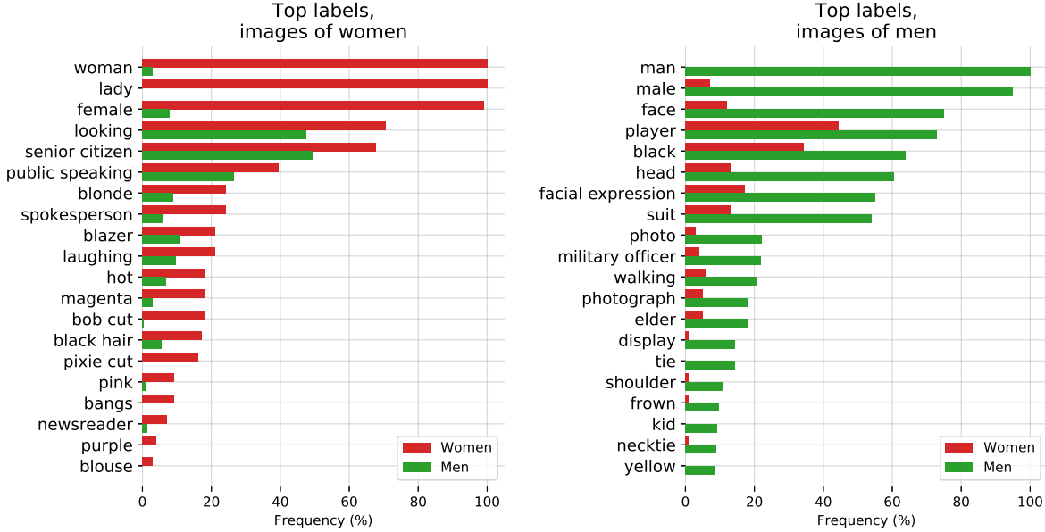
Figure 1. CLIP (ViT L/14) performance on Member of Congress images when given the combined returned label set for the images from Google Cloud Vision, Amazon Rekognition and Microsoft Azure Computer Vision. The 20 most gendered labels for men and women were identified with \chi^2 tests with the threshold at 0.5%. Labels are sorted by absolute frequencies. Bars denote the percentage of images for a certain label by gender.
