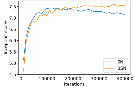
Figure 9. Inception score in CIFAR10. The results are averaged over 5 random seeds, with \alpha_g = 0.0001 , \alpha_d = 0.0001 , n_{dis} = 1 .
