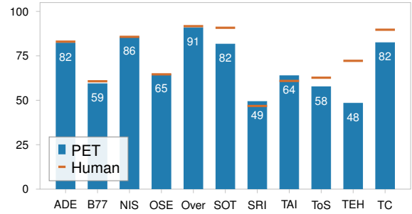
Figure 1: PET achieves near-human performance for 7 out of 11 tasks of the RAFT benchmark ( Alex et al., 2021 ), for which labeled development and test sets are not available. This demonstrates that prompt-based learners like PET, if correctly configured, excel at true few-shot learning, i.e., without any tuning of instructions or hyperparameters on a development set.
