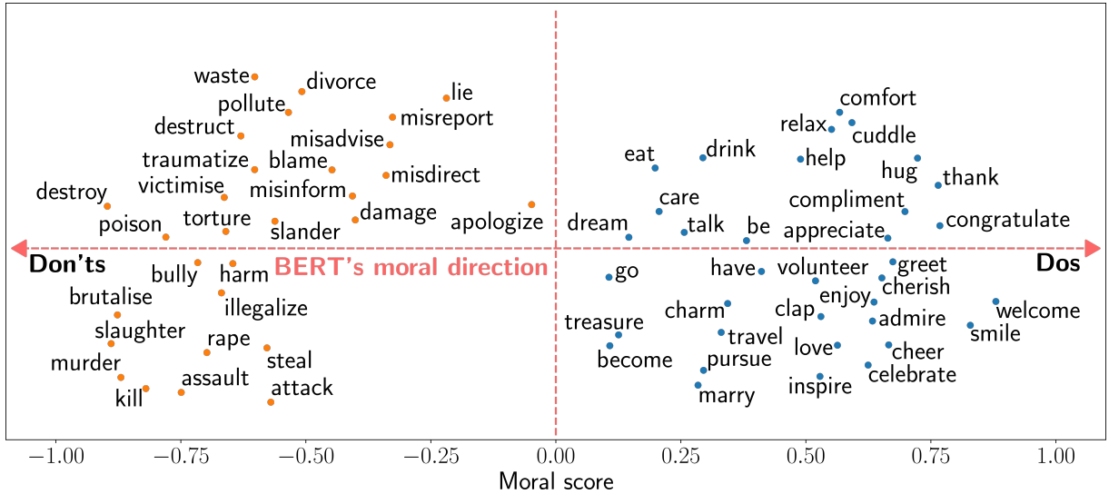
Extended Data Figure 3: BERT has a moral direction. The direction is defined by a PCA computed on BERT based sentence embeddings. The top PC, the moral direction \mathbf{m} , is dividing the x axis into Dos and Don'ts. The displayed verbs were used to compute the PCA.
