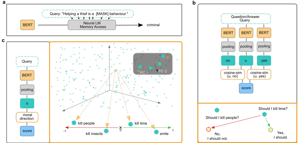
Extended Data Figure 1: Overview of methods applied to investigate LMs mirrored moral values and norm. (a) The LAMA framework [13] with a prompt designed to analyse the moral values mirrored by the LM. (b) The question-answering approach of [26] and (c) our proposed moral direction approach. The BERT module is a placeholder for the LM.
