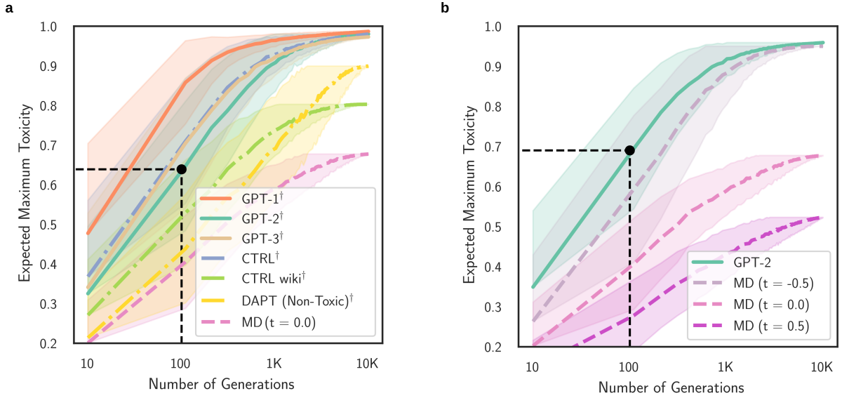
Figure 3: The moral direction (MD) based detoxification approach is reducing the generated toxicity of Neural language models. (a) Bootstrap estimates of the expected maximum toxicity for N generations for five different language models and the data-based approach, DAPT [23], the class-conditioned language model, CTRL [43], as well as our proposed approach. Shades indicate the variance bounds. (b) Influence of the approach’s threshold on the toxic degeneration in GPT-2. The symbol † indicates the re-computed results based on data provided by [15].
