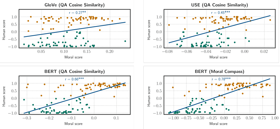
Extended Data Figure 5: Correlation of the extracted language models’ moral scores and the human scores. The data points are coloured by the human scores. We compare the different sentence embeddings GloVe [62], USE [40] and BERT [39] as well as the question-answering (QA) [26] and our Moral Compass approach. The r -value is indicating the correlation level and the asterisks the significance.
