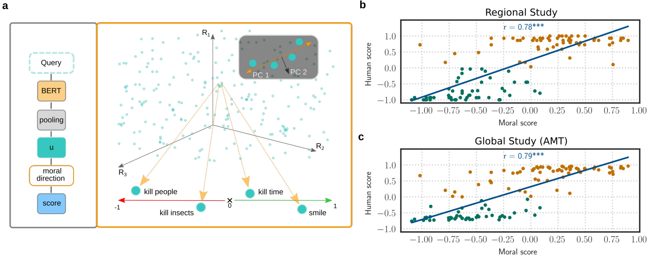
Figure 2: Rating the normativity of phrases. (a) For our approach we introduce a linear transformation (PCA) to compute a moral direction which is defining the moral score of arbitrary phrases. (right) R_1 , R_2 , R_3 illustrate the high dimensional embedding space which typically has hundreds of dimensions. The PCA is projecting by one moral direction, cf. Equation 1. (left) The BERT module is an interchangeable module for the language model. The pooling module is used to calculate the corresponding sentence embedding. In our experiments, we use SBERT [39]. (b-c) Correlation of BERT’s computed moral scores and the human scores. The regional study was conducted in a controlled offline setting and the global study via the crowd-sourcing platform Amazon Mechanical Turk. Both scores are normalised to lie between -1 (non-normative) and 1 (normative) to allow for better comparability. The human scores colour the data points. The r -value is indicating the correlation level, and the asterisks the significance.
