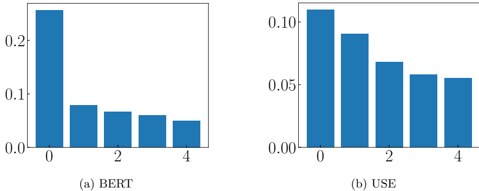
Extended Data Figure 4: PCA variance explained.
