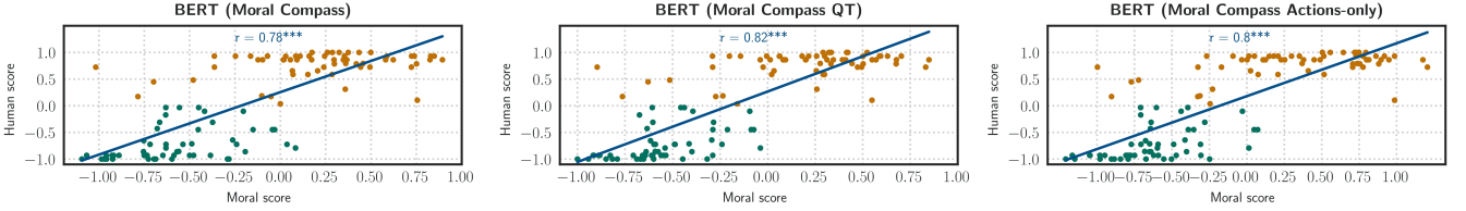
Extended Data Figure 6: Correlation of the extracted language models’ moral scores and the human scores. The data points are coloured by the human scores. Here, we compare querying the Moral Compass approach with the same phrases the user study was conducted on (left), using the average embeddings by prompting the actions into the question template (middle) and querying the raw actions (right). The r -value is indicating the correlation level and the asterisks the significance.
