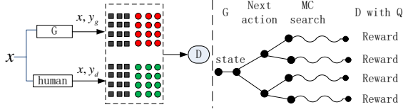
Figure 1: The Illustration of the proposed BR-CSGAN. Left: D is trained over the real sentence pairs translated by the human and the generated sentence pairs by G. Note that D is a conditional discriminator. Right: G is trained by policy gradient where the final reward is provided by D and Q.
