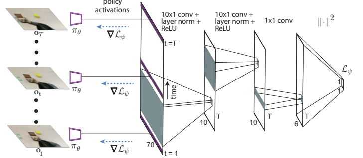
Fig. 2. Visualization of the learned adaptation objective, which uses temporal convolutions to integrate temporal information in the video demonstration.
