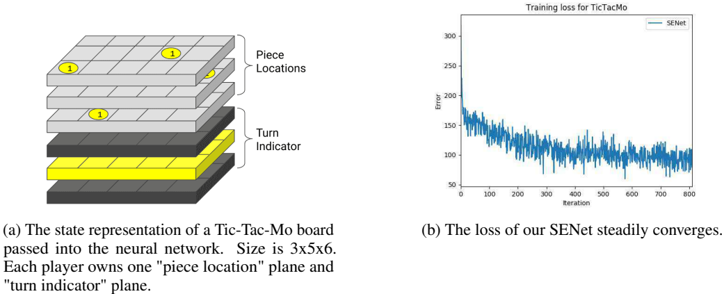
Figure 2: State representation and loss curve for Tic-Tac-Mo.
