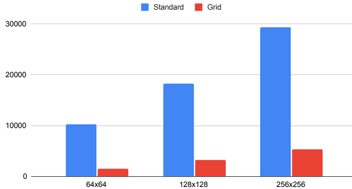
Figure 7: Memory cost comparison between standard self-attention and grid self-attention
