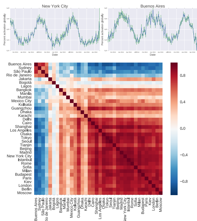
Figure 9: Top: Mean major color frequency for the color white for two cities highlighting flipped behavior between the Northern and Southern Hemisphere. Means are computed by aggregating measurements per 1 week intervals and error bars indicate a 95% confidence interval. Bottom: Pearson's correlation coefficients for the mean prediction score of the color white across all pairs of major world cities. Cities have been ordered by latitude to highlight the relationship between the northern and southern hemispheres and their relationship to the seasonal trend of the color white.
