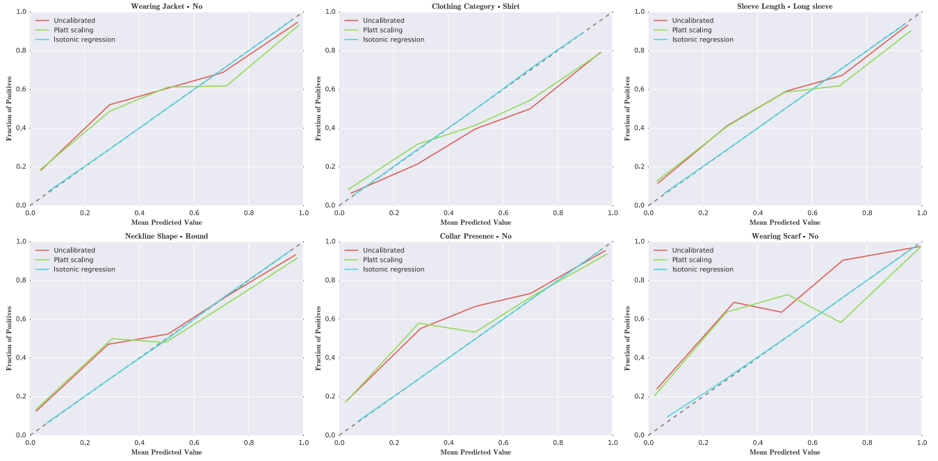
Figure 5: Reliability curves for several clothing attributes. A well-calibrated reliability curve has fraction of positives equal to mean predicted value. Neural networks tend to produce well-calibrated probabilities, but significant improvement is made using Isotonic regression for additional calibration.
