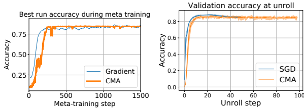
Figure 7. Using CMA to learn best non-differentiable accuracy objective, against gradient based meta training. Left : meta-training trajectory right : fully trained genome learning MNIST. Both methods show best run out of 8.
