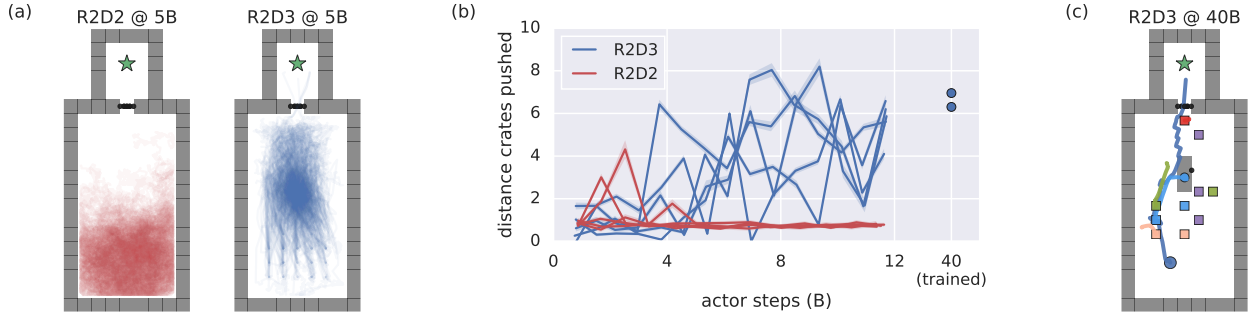
Figure 7 | Guided exploration behavior in the Push Blocks task. (a) Spatial pattern of exploration behavior at ~5B actor steps (reward-driven learning kicks off for R2D3 only after ~20B steps). Overlay of agent’s trajectories over 200 episodes. Blocks and sensors are not shown for clarity. R2D2 appears to follow a random walk. R2D3 concentrates on a particular spatial region. (b) Interactions between the agent and blocks during the first 12B steps. Each line shows a different random seed. R2D2 rarely pushes the blocks. (c) Example trajectory of R2D3 after training, showing the agent pushing the blue block onto the blue sensor, then going to collect the apple reward (green star).
