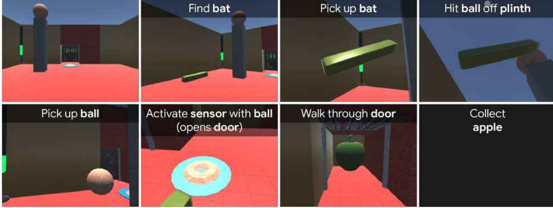
Figure 3 | High-level steps necessary to solve the Baseball task. Each step in this sequence must be completed in order, and must be implemented by the agent as a sequence of low level actions (no option structure is available to the agent). The necessity of completing such a long sequence of high level steps makes it unlikely that the task will ever be solved by random exploration. Note that each step involves interaction with physical objects in the environment, shown in bold.
