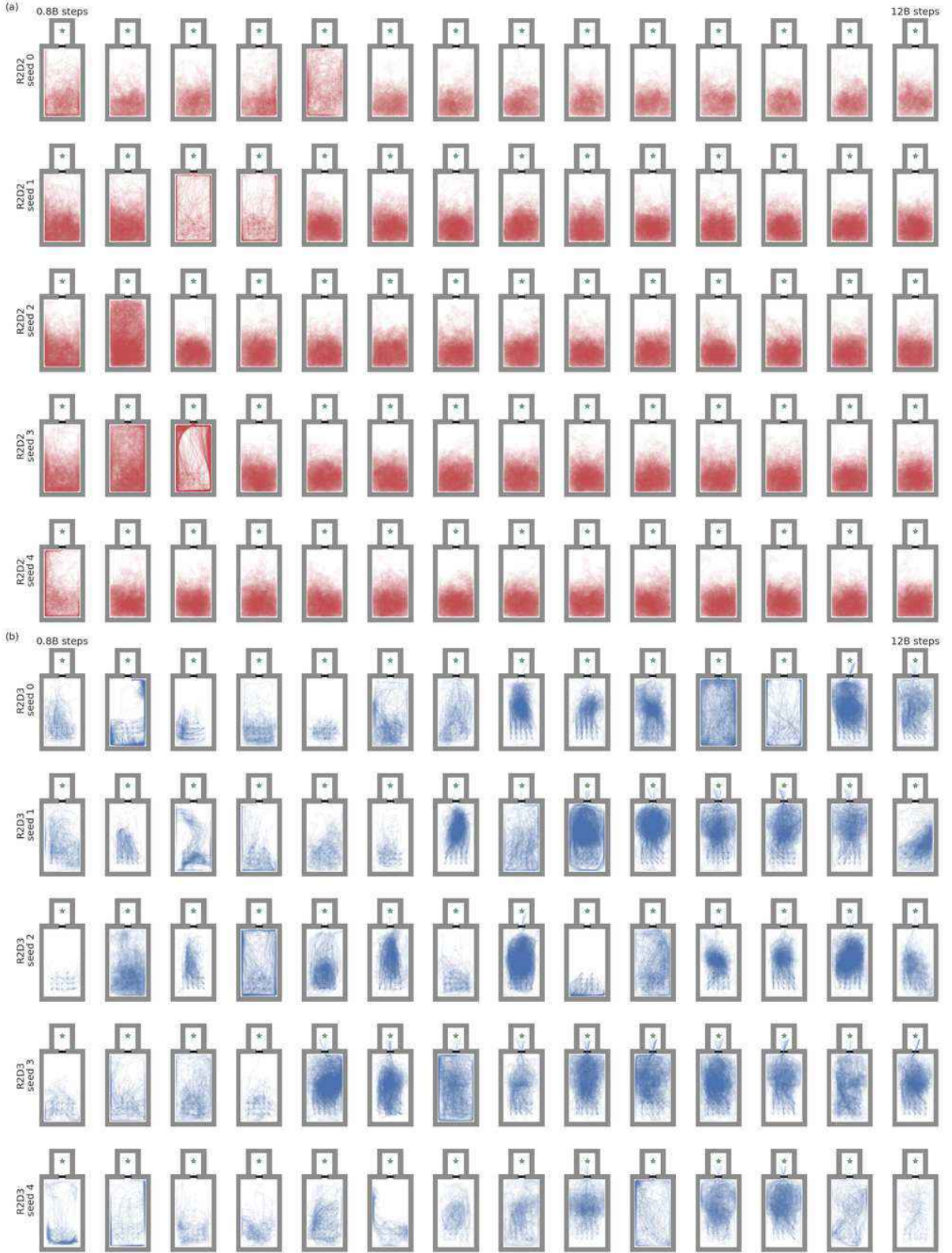
Figure 12 | Further detail of guided exploration behavior in the Push Blocks task (as in Figure 7). (a) Spatial pattern of exploration behavior for the R2D2 agent over the course of \sim 12B steps of training. Each row shows a different random seed; the number of training steps increases from the leftmost column to the rightmost column. There is little variation in how the policy manifests as explorative behavior across seeds and training time. (b) As in (a), for R2D3. Given demonstrations, the policies now show substantial variation across seeds and training time.
