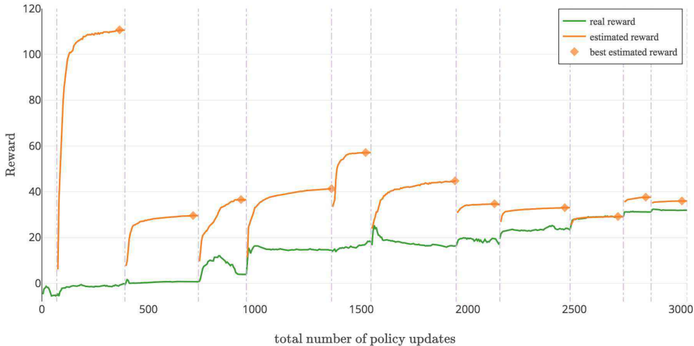
Figure 5: Predicted and real performances during the training process using our approach with one model instead of an ensemble in Swimmer. The policy overfits to the dynamics model which degrades the real performance.
