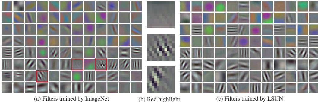
Figure 6: Comparison of learned filters. We train AlexNet with our object images and compare the first level filter with ImageNet. We observe that the filter pattern learned with our data is cleaner, while the filters from ImageNet are noisier, as highlighted in (b).
