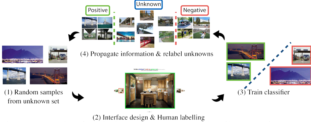
Figure 1: An overview of our pipeline. To annotate a large number of images, we first randomly sample a small subset (1) and label them through crowdsourcing using our Amazon Mechanical Turk interface(2). This small labeled subset is then utilized to train a binary classifier with deep learning feature (3). Then, we run the binary classifier on the unlabeled images. The images with high or low scores are labeled as positive or negative automatically, while the images ambiguous to the classifier are fed into the next iteration as the unlabeled images (4). The pipeline runs iteratively until the number of images remaining in the unknown set is amenable to exhaustive labeling.
