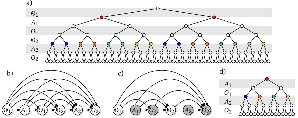
Figure 3 | Stochastic process over the binary random variables \Theta_1, A_1, O_1, \Theta_2, A_2, O_2 representing interactions between Nature (choosing \Theta 's and O 's) and the agent (choosing A 's). The interactions can be represented as a game in extensive form (Panel a) or as a causal Bayesian network (Panel b). In the partially observable case the \Theta 's are hidden moves by Nature, which create information sets (=collection of indistinguishable states) for the agent. These are shown explicitly in (a) as nodes sharing the color which reduce the game to (d). Panel (c) shows the graph resulting from treating actions as interventions. Panel (d) shows the game representing the marginal interaction process that the agent experiences when Nature makes hidden moves. This game is causally insufficient for evaluating the effects of interventional actions.
