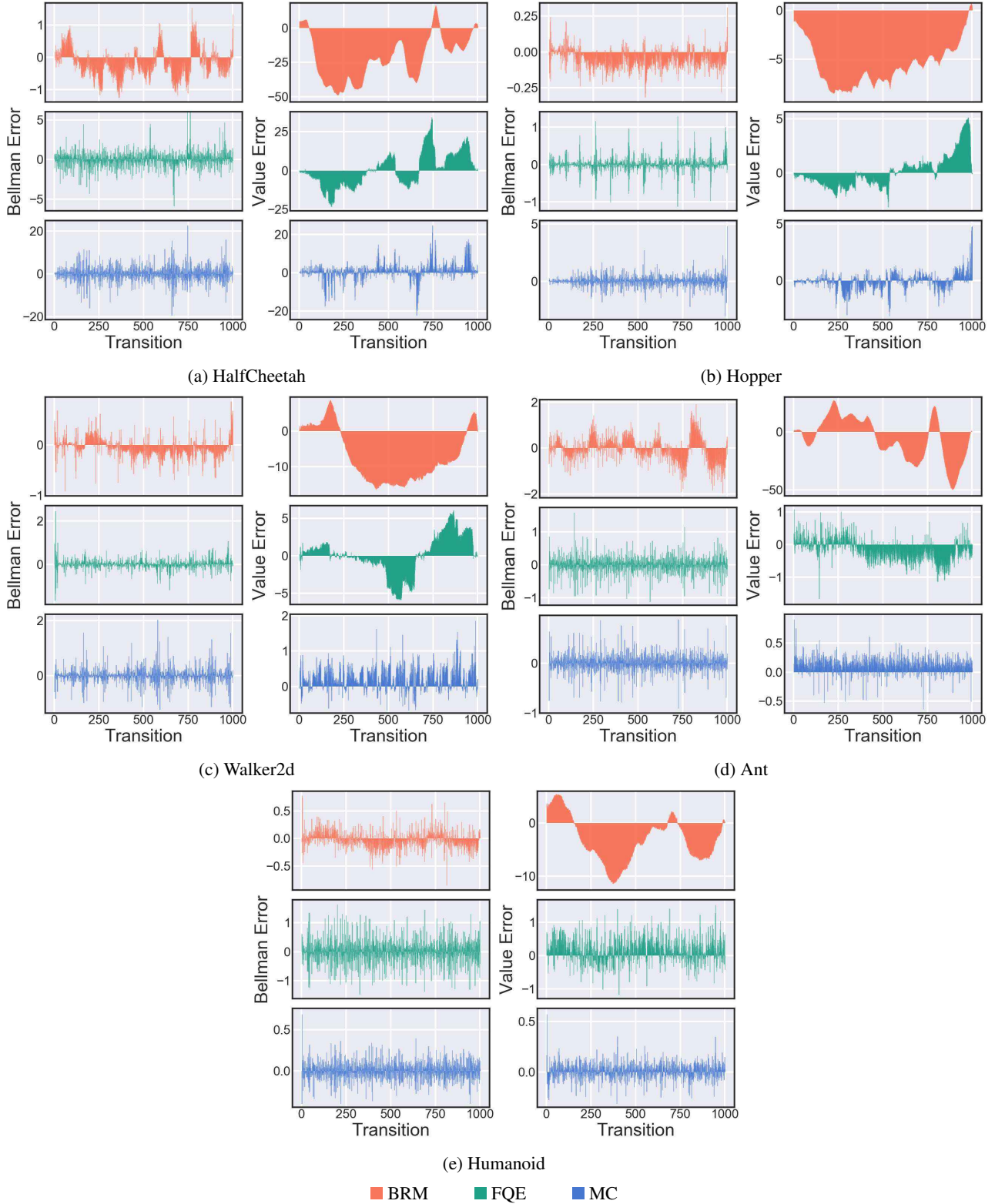
Figure 4: Does bias explain the non-correspondence between Bellman error and value error? We train value functions over a single on-policy trajectory (1000 transitions, with termination). As a result, every relevant transition is contained in each dataset. We display the Bellman error (left) and unnormalized value error (right) for every transition in the trajectory. Visually, we can see that the clusters of similar value error (size and direction) can cause lower magnitude Bellman error for ■ BRM and ■ FQE.
