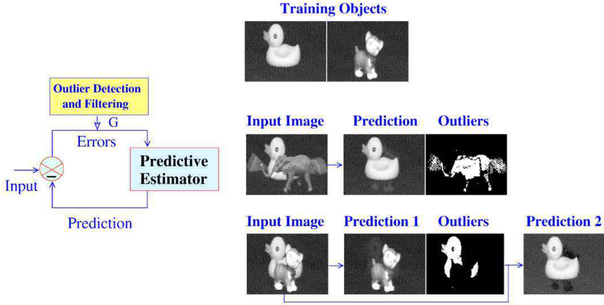
Figure 4. Robust Predictive Coding and Attention. (Left) The robust predictive coding model utilizes a gain or gating term G to modulate the prediction errors before they are fed to the predictive estimator network that estimates the state vector \mathbf{r} . This allows the network to filter out any outliers dynamically as a function of the current top-down hypothesis, allowing the network to “focus attention” and test its hypothesis. (Right) The top row shows images of two objects the network was trained on. The middle row illustrates how the network can filter out occluders and background objects as outliers, recovering an estimate of a training object (the duck). The bottom row shows how, when presented with an image containing both training objects, the network can sequentially focus and recognize each object.
