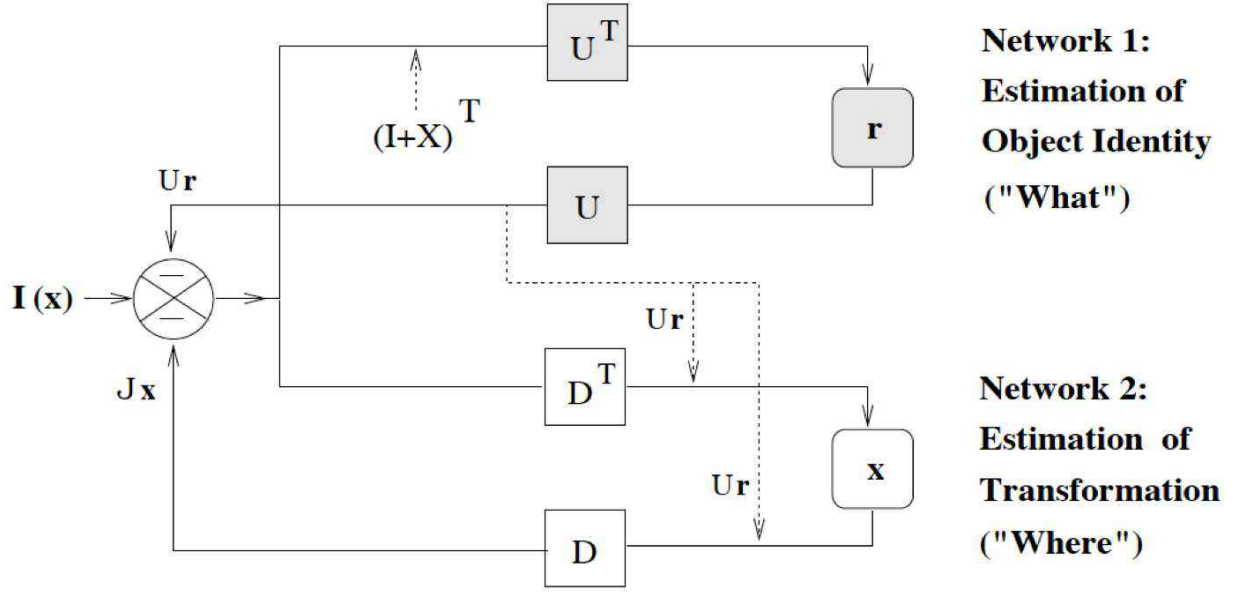
Figure 5. What-Where Predictive Coding Networks: Two networks jointly minimize prediction error: one network estimates object features/identity ("What") while the other estimates transformations ("Where") relative to a canonical representation.
