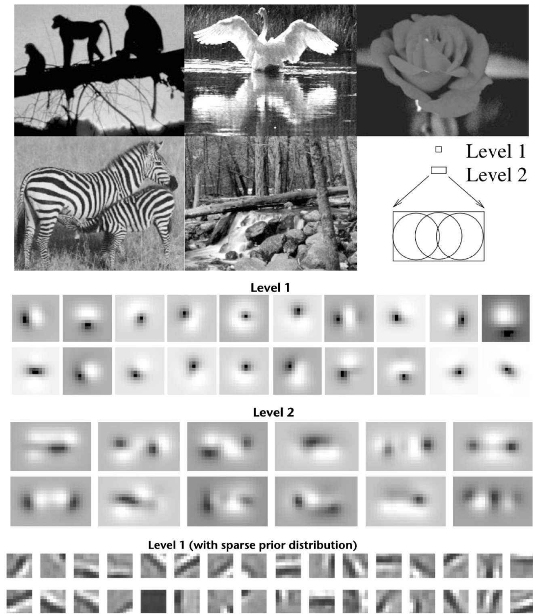
Figure 6. Emergence of visual cortex-like receptive fields in the hierarchical predictive coding model. Adapted from Rao & Ballard, 1999. (Top) Natural images used for training the hierarchical model. Several thousand natural image patches were extracted from these five images. The bottom-right corner shows the size of Level 1 and Level 2 receptive fields relative to the natural images. (Middle two panels) Level 1 and Level 2 feedforward synaptic weights (rows of U^T ) learned from the natural images using a Gaussian prior. Values can be zero (always represented by the same gray level), negative (inhibitory, black regions), and positive (excitatory, bright regions). These weights resemble centered oriented Gabor-like receptive fields in Level 1 and in Level 2, various combinations of the synaptic weights in Level 1. (Bottom panel) Localized
