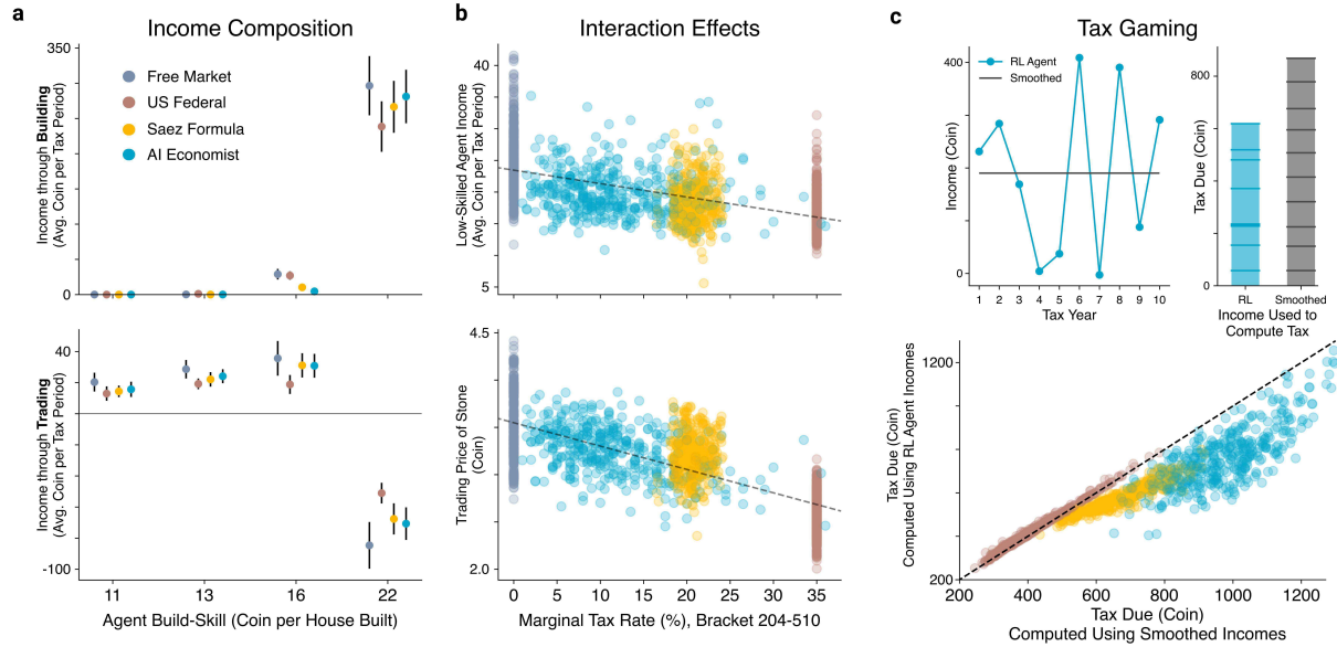
Figure 6: Specialization, interactions, and tax gaming in the 4-agent Open-Quadrant Gather-Trade-Build environment. a , Average net income from building (a, top) and trading (a, bottom) of each agent. Negative values denote net expenditure. b , The income of the two lowest build-skill agents (b, top) and average trading price (b, bottom) decrease as the tax rate in the higher 204-510 tax bracket increases, even though the agents’ incomes are below the cutoff for this bracket. Hence, the trading behavior of high-skilled agents affects the income of the low-skilled agents. The standard definition of elasticity does not capture this interaction effect. c , RL agents learn to strategize across each of the 10 tax years, lowering their total payable tax compared to a smoothed strategy that earns the same, average income in each year: the top panels illustrate this for a single episode; the bottom panel shows the saving relative to a smoothed income across all episodes used in the analysis. We do not observe this tax gaming under the progressive US Federal tax schedule.
