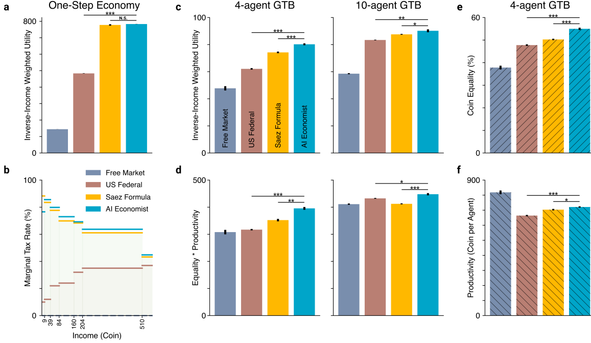
Figure 3: Quantitative results in a one-step economy and the Open-Quadrant Gather-Trade-Build environment. a-b, The results of the AI Economist and the Saez tax are highly consistent in the one-step economy, both in terms of utilitarian social welfare (a) and the tax schedule (b). c-d, In the Gather-Trade-Build environment (GTB) with 4 and 10 agents, the AI Economist outperforms baselines when optimizing the utilitarian social welfare objective (c) and when optimizing the equality-times-productivity objective (d). e-f, Overall coin equality (e) and average productivity (f) achieved by each tax model in the 4-agent Open Quadrant scenario. Each bar represents the average end-of-training metrics over 10 random seeds (5 for the one-step economy), with error bars denoting standard error. Asterisks indicate a statistically significant difference at an \alpha level of 0.05 (*), 0.001 (**), or 0.00001 (***). N.S. denotes not statistically significant ( p > 0.05 ). All social welfare, productivity, and equality differences between the AI Economist and baselines are statistically significant, except for the difference in social welfare between the AI Economist and the Saez tax in the one-step economy (a).
