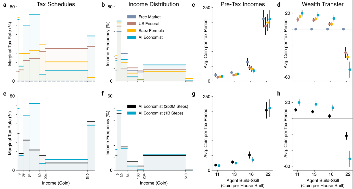
Figure 5: Comparison of tax policies in the 4-agent Open-Quadrant Gather-Trade-Build environment. a , Average marginal tax rates within each tax bracket. b , Frequency with which agent incomes fall within each bracket. c , Average pre-tax income of each agent (sorted by build-skill) under each of the tax models. d , Average wealth transfer resulting from taxation and redistribution. e-h , Same as a-d, comparing the AI Economist from early during training (250 million training samples) versus at the end of training (1 billion training samples). Dots denote averages and error bars denote standard deviation across episodes.
