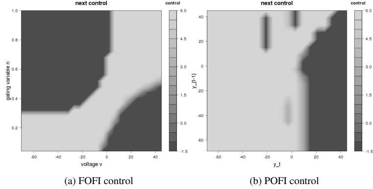
Figure 1: Long term controls of FOFI and POFI for the parameter g_{Ca} . The FOFI plot gives the control to use, given a certain position in state space. The POFI control will depend on the last two observations and the last control, but fixing the last control as, for example, I_{t-1} = 6 one can plot which control to use given combinations of the last two observations.
