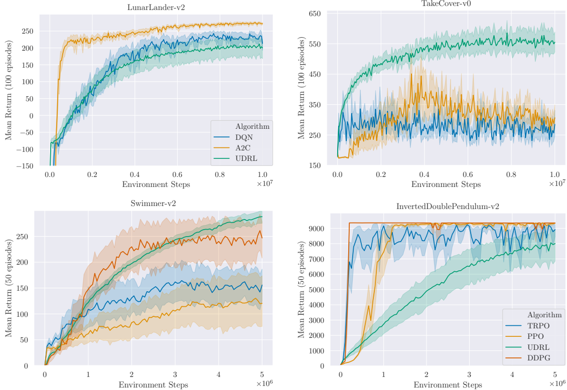
Figure 3. Results on tasks with discrete-valued actions (top row) and continuous-valued actions (bottom row). Solid lines represent the mean of evaluation scores over 20 runs using tuned hyperparameters and experiment seeds 1–20. Shaded regions represent 95% confidence intervals using 1000 bootstrap samples. \mathcal{T}\mathcal{D} is competitive with or outperforms traditional baseline algorithms on all tasks except InvertedDoublePendulum-v2.
