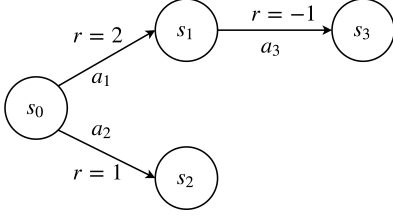
Figure 2: A toy environment with four states.
