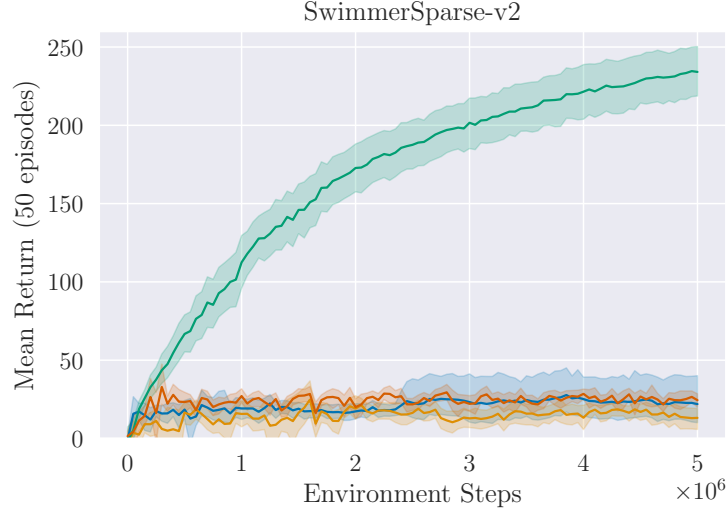
Figure 6: Results on SwimmerSparse-v2. Blue: TRPO, Yellow: PPO, Red: DDPG, Green: TD.
