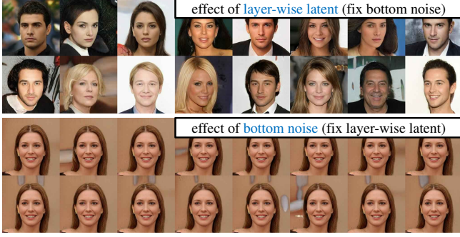
(a) With the subspace models (EigenGAN), major variations are captured by the layer-wise latent variables.
