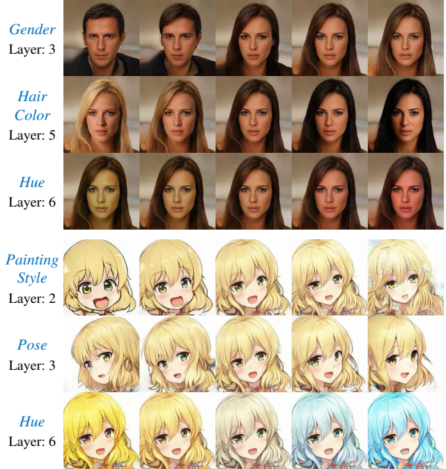
Figure 1. Example of interpretable dimensions learned by EigenGAN. The smaller the index, the deeper the layer.
