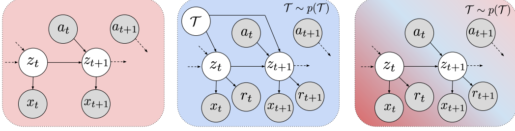
Figure 2: (a) : When only partial observations of the underlying state are available, latent dynamics models can glean state information \mathbf{z}_t from a history of observations. (b) : Meta-RL considers a task distribution where the current task \mathcal{T} is an unobserved variable that controls dynamics and rewards. (c) : We interpret \mathcal{T} as part of \mathbf{z}_t , allowing us to leverage latent dynamics models for efficient image-based meta-RL.
