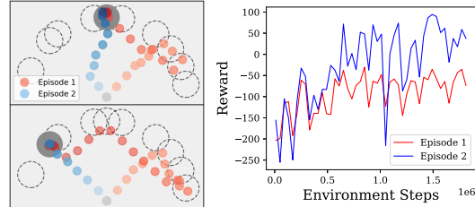
Figure 15: Image-based 2D navigation with reward given after finding the right goal: (Left) trajectory traces of meta-learned exploration finding goal in Episode-1 (red) and going directly there in Episode-2 (blue). (Right) higher rewards in episode-2 show preservation of information across episodes.
