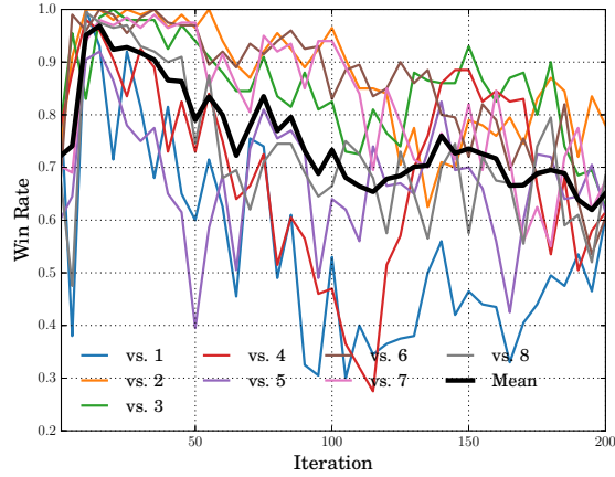
Figure 12: The win rate for PBT against all 8 baselines, this time with ML value networks instead of a single value output.
