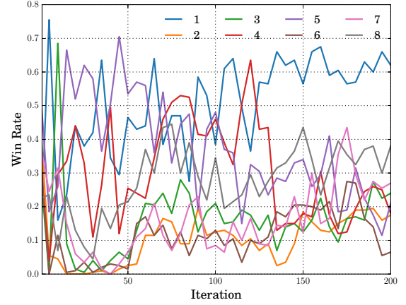
Figure 10: The round-robin results of 8 baseline versions with ML value networks. The win rates shown are the minimum win rates.
