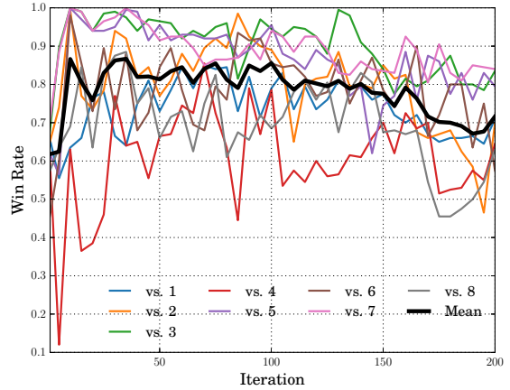
Figure 3: The win rate for PBT against all 8 baselines. Note that each line refers to PBT’s win rate; a value of 0.5 or higher indicates that PBT is stronger.
