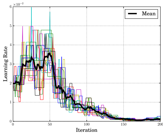
Figure 13: The learning rate curve during training for ML value networks.
