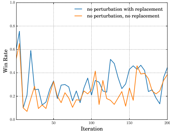
Figure 6: The win rates for the two ablation methods against the PBT method.
