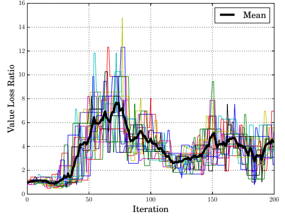
Figure 5: The value loss ratio curve during training. The colored lines depict the settings for different agents in the population. The solid black line depicts the mean.
