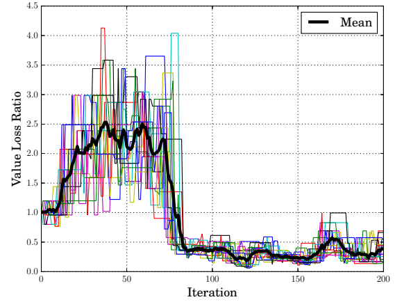
Figure 14: The value loss ratio curve during training for ML value networks.
