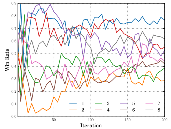
Figure 11: The round-robin results of 8 baseline versions with ML value networks, where the average win rates are shown.
