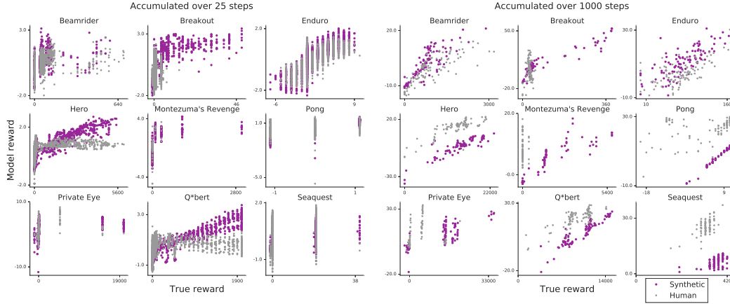
Figure 8: True vs. model reward accumulated in sequences of 25 (left) and 1000 (right) agent steps. Magenta and gray dots represent the model learned from synthetic (demos + pr. + autolabels in Figure 1) and human preferences, respectively. A fully aligned reward model would have all points on a straight line. For this evaluation, the agent policy and reward model were fixed after successful full-schedule training (in the case of synthetic feedback we chose the most successful seed; in the case of human feedback, there was no choice, only one run was available).
