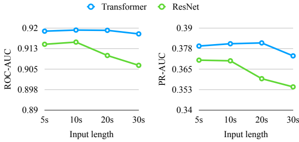
Figure 2: Performance with different input lengths.
