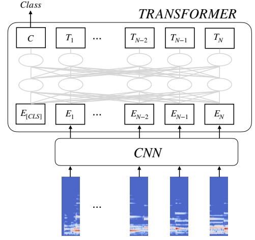
Figure 1: Proposed Music Tagging Transformer.
