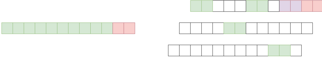
Figure 4: The conventional unsupervised causal modeling (left) vs. our modified MARGE (right). Note that each block consists of multiple tokens. If a model tries to predict the tokens in last two blocks (red), the attention is paid to the past tokens in the red region as well as the tokens in context (green). The modified MARGE reads the immediate context (purple) to find the relevant parts across the dataset and the past of the current sample in order to use them as a context.
