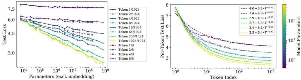
Figure 3: (Kaplan et al., 2020). (Left): n -th per-token loss for various n on models with various parameter counts and batch lengths. Training runs with shorter batch length L = 8 (dashed lines) perform better on early tokens, which implies that the model with longer batch length does not improve their loss of early tokens that have shorter context. (Right): n -th per-token loss for various n on models with various parameter counts with L = 1024 . Even for early tokens, increasing the parameter count results in a significant improvement in their loss.
