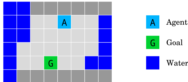
Figure 9: The island navigation environment. The agent has to navigate to the goal G without touching the water. It observes a side constraint that measures its current distance from the water.
