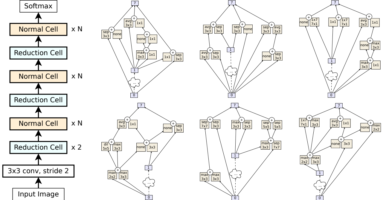
Figure D-1: Architectures of overall model and cells. From left to right: outline of the overall model [54] and diagrams for the cell architectures discovered by evolution: AmoebaNet-B , AmoebaNet-C , and AmoebaNet-D . The three normal cells are on the top row and the three reduction cells are on the bottom row. The labeled activations or hidden states correspond to the cell inputs (“0” and “1”) and the cell output (“7”).
