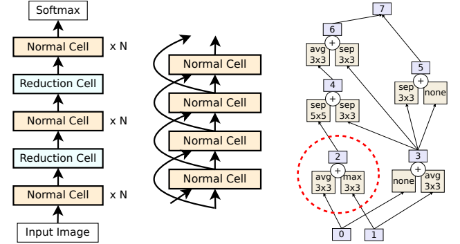
Figure 1: NASNet Search Space [54]. LEFT: the full outer structure (omitting skip inputs for clarity). MIDDLE: detailed view with the skip inputs. RIGHT: cell example. Dotted line demarcates a pairwise combination.
