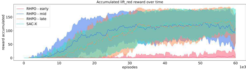
Figure 5 | Learning curves for hierarchical skill learning of lift_red using SelMo auxiliary policies in the JACO environment. The SAC-X baseline uses auxiliary reward functions {reach,move}_red . Each RHPO run uses five randomly sampled SelMo policies from the respective intervals as auxiliary skills (cf. section 4.2). Mean and standard deviation are plotted for five random seeds for each model and the plot is smoothed with an exponential filter of \sigma = 1.5 .
