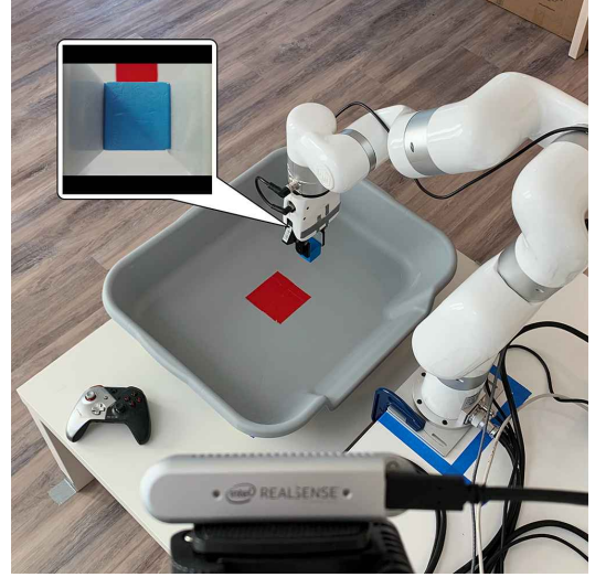
Fig. 1: The Framework for Efficient Robotic Manipulation (FERM) enables robotic agents to learn skills directly from pixels in less than one hour of training. Our setup requires a robotic arm, two cameras, and a joystick to provide 10 demonstrations.
