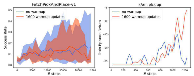
Fig. 11: Unsupervised pretraining ablation on simpler tasks. In both pick up and simulated pick and place, warming up the encoder doesn't introduce significant difference to the RL training performance. The real robot plot (right) is smoothed using a Gaussian kernel for better visibility.
