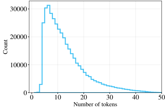
Figure 6. Sentences length distribution. Queries length is measured in number of tokens.
