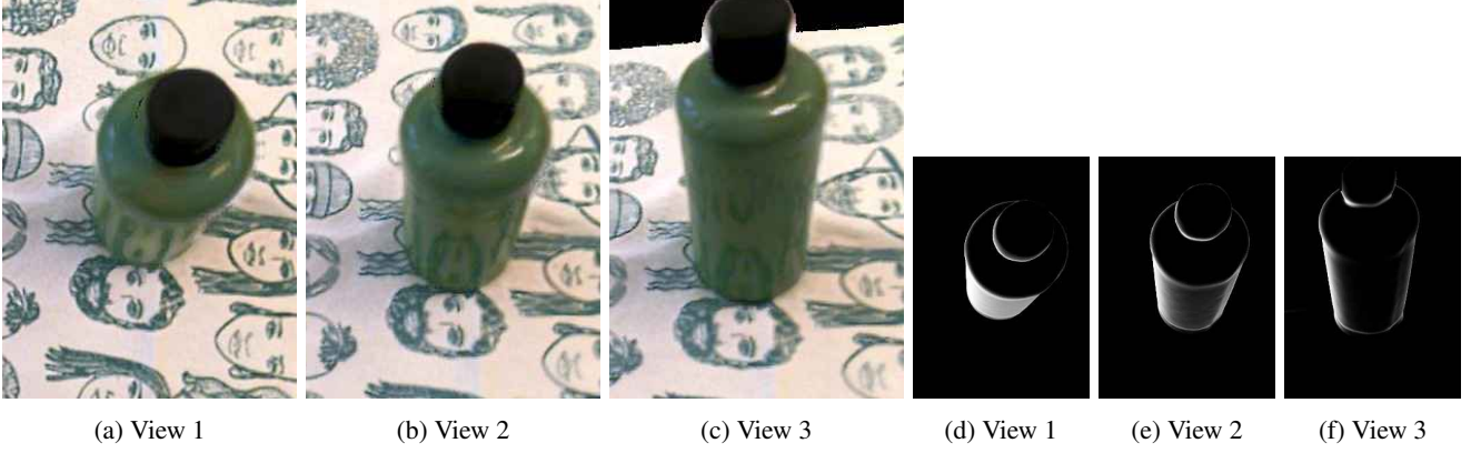
Figure 14: Demonstration of the Fresnel effect. The intensity of specular highlights tends to be amplified at slant viewing angles. We show three different views (a,b,c) for a glossy bottle, each of them generated by our neural rendering pipeline and presenting different viewing angles with respect to the bottle. Notice that the neural rendering correctly amplifies the specular highlights as the viewing angle gets closer to perpendicular with the surface normal. Images (d,e,f) show the computed Fresnel coefficient (FCI) (see Sec. 6.1) for the corresponding views. These images are given as input to the neural-renderer that subsequently use them to simulate the Fresnel effect. Best viewed digitally.
