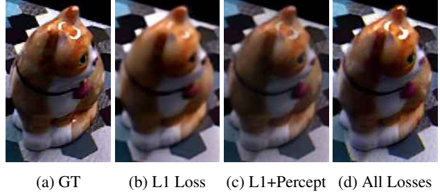
Figure 11: Effects of loss functions on neural-rendering. The specular highlights on the forehead of the Labcat is expressed weaker than it actually is when using L1 or perceptual loss, likely due to geometric and calibration errors. The highlight is best expressed when the neural rendering pipeline of Sec. 6 is trained with the combination of L1 , perceptual, and adversarial loss.
