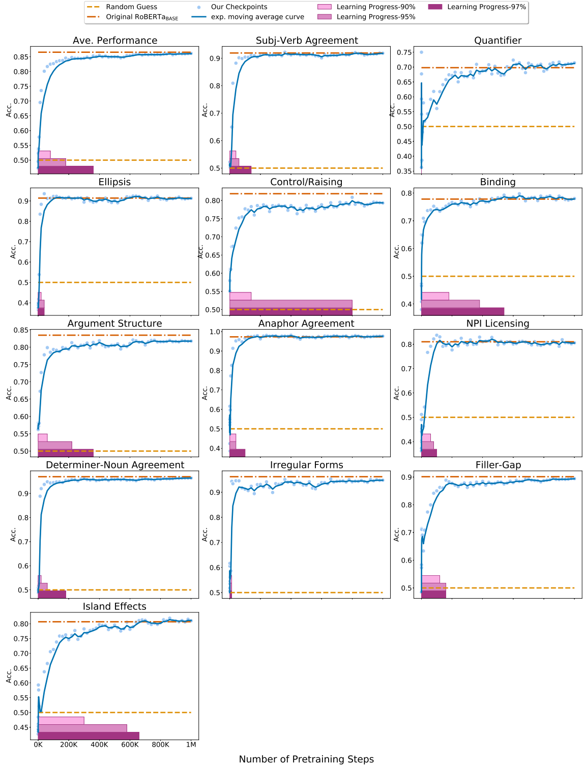
Figure 5: Complete results of BLIMP (Linguistics) in Figure 1, plotted in the same format.
