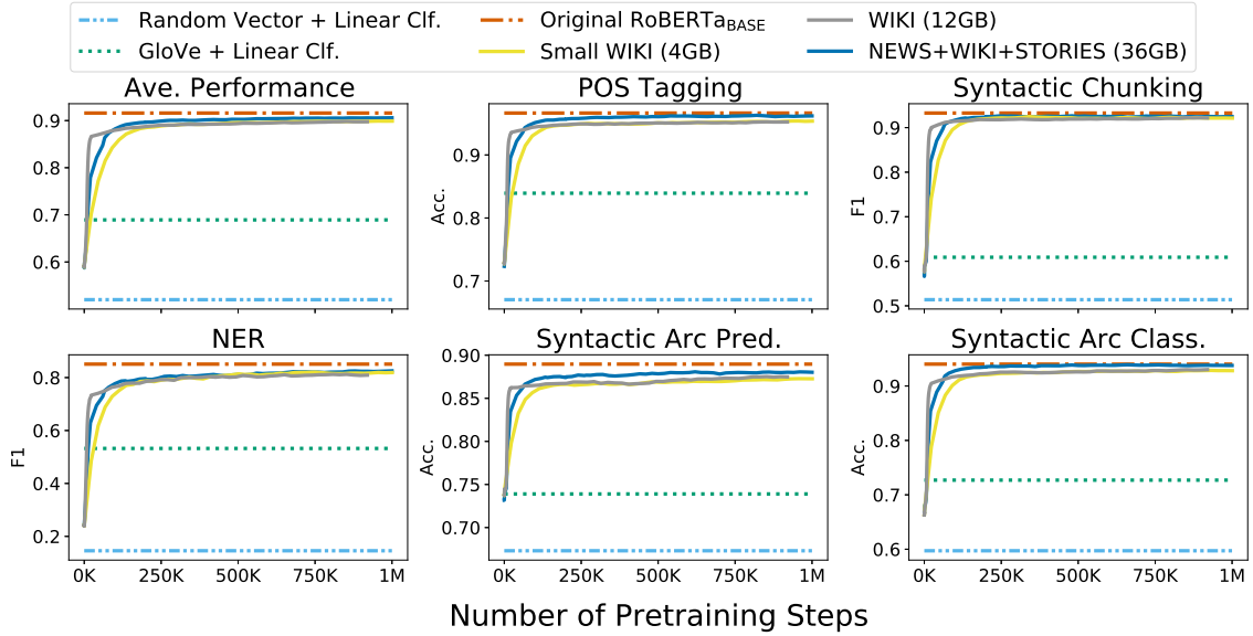
Figure 13: Complete results of LKT (Linguistics) on different corpus sizes. Following Fig. 1, every line in plots are smoothed using exponential moving average with coefficient 0.5. Average performance is calculated from all included tasks in this plot.
