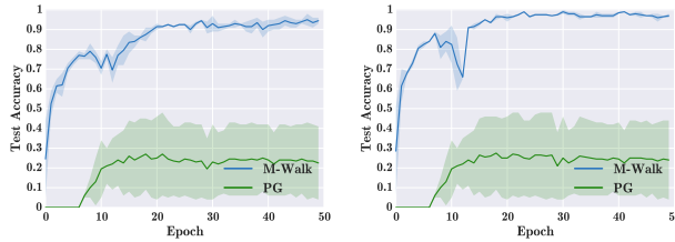
(a) Test Beam / Rollout = 128 (b) Test Beam / Rollout = 300
