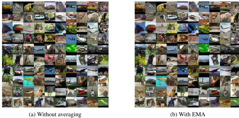
Figure 10: Generation for STL-10 dataset after 500k iterations.
