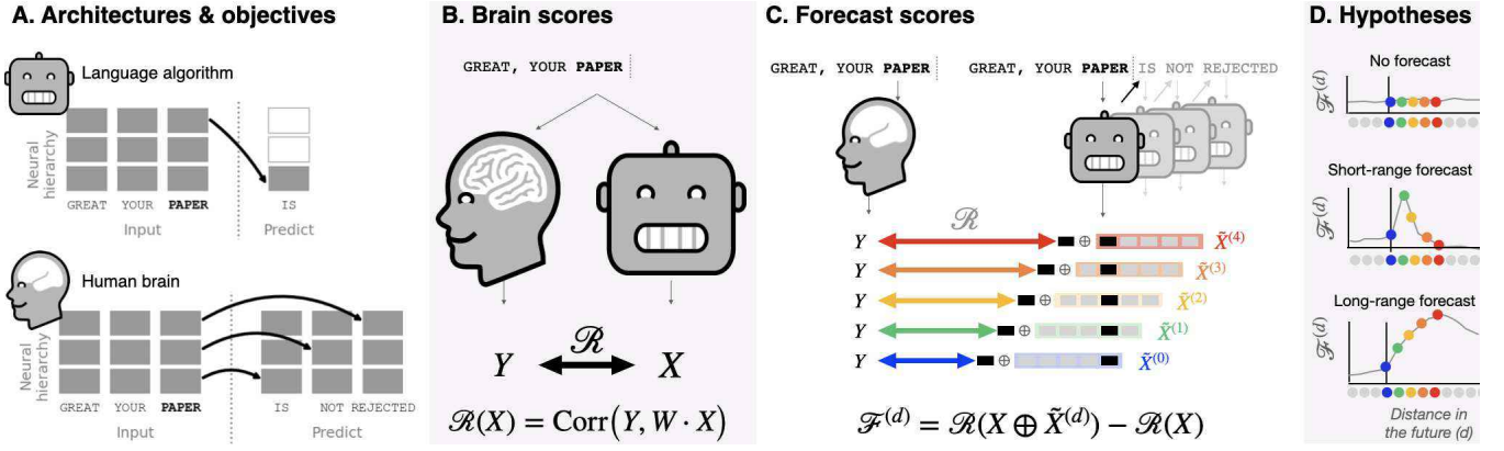
Fig. 1. Approach. A. Deep language algorithms are typically trained to predict words from their close contexts. Unlike these algorithms, the brain makes, according to predictive coding theory, (i) long-range and (ii) hierarchical predictions. B. To test this hypothesis, we first extract the fMRI signals of 304 subjects each listening to \approx 70 min of short stories ( Y ) as well as the activations of a deep language algorithm ( X ) input with the same stories. We then quantify the similarity between X and Y with a “brain score”: a Pearson correlation \mathcal{R} after an optimal linear projection W (Methods D). C. To test whether adding representations of future (or predicted, see Figure S6) words improves this correlation, we concatenate ( \oplus ) the network’s activations ( X , depicted here as a black rectangle) to the activations of a “forecast window” ( \tilde{X} , depicted here as a colored rectangle). We use principal component analysis to reduce the dimensionality of the forecast window down to the dimensionality of X . Finally, \mathcal{F} quantifies the gain of brain score obtained by enhancing the activations of the language algorithm to this forecast window. We repeat this analysis with variably distant windows ( d , Methods E). D. A flat forecast score across distances would indicate that forecast representations do not make the algorithm more similar to the brain (top). By contrast, a forecast score peaking at d > 1 (bottom) would indicate that the model lacks brain-like forecast. The peak of \mathcal{F}^{(d)} indicates how far off in the future the algorithm would need to forecast representations to be most similar to the brain.
