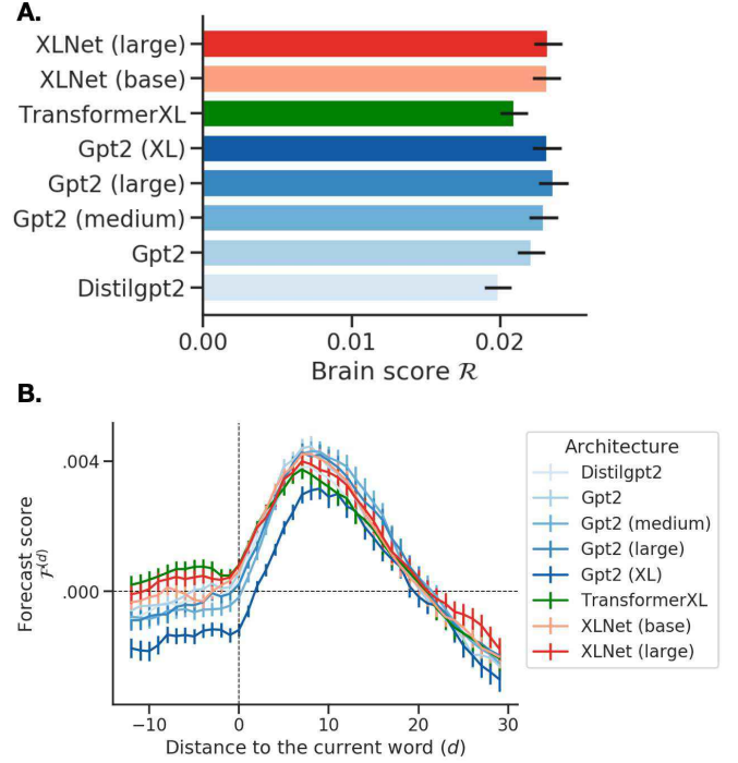
Fig. S5. Generalisation to other architectures. A. Brain scores (cf. Figure 1B, Methods D) of eight transformer models, based on XLNet (67), TransformerXL (68) and GPT-2 (2) architectures. We use the pre-trained models from Huggingface and proceed similarly as with GPT-2 (Methods C). Brain scores are averaged across voxels and subjects, error bars are the standard errors of the mean across subjects. B. Same as Figure 2D for the eight transformer architectures.
