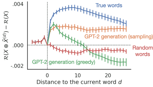
Fig. S6. Controls. Forecast scores for different types of forecast representations \tilde{X} . Here, we use a growing window analysis: \tilde{X}^{(d)} is the concatenation of the activations of |d| future ( d > 0 ) or past ( d < 0 ) words; the size of the window thus varies with the distance. The forecast score is the gain in brain score when concatenating the forecast window (cf. Eq. (3)). In blue, \tilde{X} is built out of the true words of the story. In red, \tilde{X} is built out of randomly picked words from all stories. In green and orange, \tilde{X} is built out of words generated by GPT-2. Precisely, GPT-2 is input with the current word and its previous context, and we use greedy (green) and sampling (orange) decoding schemes to generate a sequence of expected words. For simplicity, when d < 0 , \tilde{X} is the concatenation of d true past words. When d > 0 , \tilde{X} is the concatenation of d future words (either true, generated or random words).
