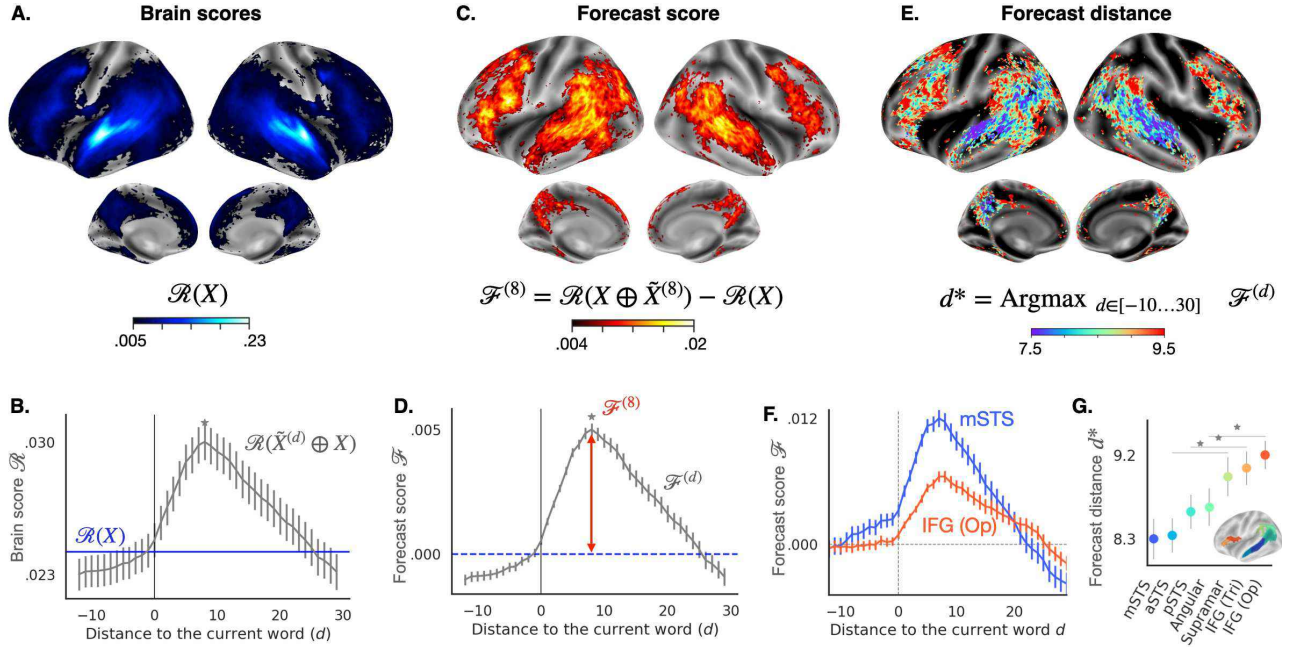
Fig. 2. Long-range forecasts in the brain. A. The “brain score” ( \mathcal{R} , Figure 1B, Methods D), obtained with GPT-2, for each subject and each voxel, and here averaged across subjects ( n=304 ). Only the voxels with significant brain scores are color-coded. B. Average (across voxels) brain scores obtained with GPT-2 with (grey) or without (blue) forecast representations. The average brain score peaks at d^* = 8 (grey star). C. For each voxel, the average (across subjects) “forecast score” \mathcal{F}^d , i.e. the gain in brain score when concatenating the activations of GPT-2 with a forecast window \tilde{X}^{(8)} . Only the voxels with significant forecast scores are color-coded. D. Average (across voxels) forecast scores for different distance d . E. Distance that maximizes \mathcal{F}^d , computed for each subject and each voxel, and denoted d^* . This “forecast distance” reveals the regions associated with short- and long-range forecasts. Regions in red and blue are associated with long-range and short-range forecasts, respectively. We only display the voxels with a significant average peak ( \mathcal{F}^{d^*} - \mathcal{F}^0 , d^* = 8 , cf. Methods G). F. Same as D. but for two selected regions of the brain: the middle superior temporal sulcus (mSTS) and the pars opercularis of the inferior frontal gyrus (IFG-Op). G. Forecast distance of seven regions of interest, as computed for each voxel of each subject and then averaged within the selected brain regions. For all panels, the error bars are SEM across subjects. All brain maps are thresholded at p < .01 , as assessed with a FDR-corrected two-sided Wilcoxon test across subjects.
