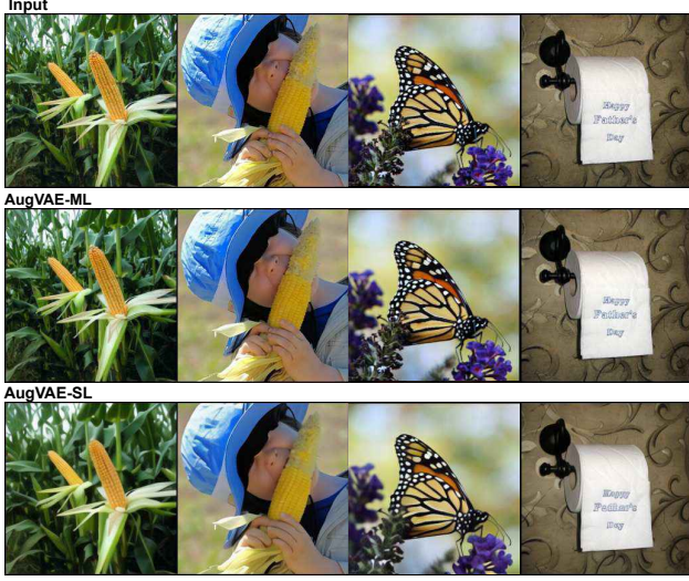
Figure 3. Comparison of input images ( top ), reconstructions from multi-level (hierarchical) feature-augmented variational autoencoder (AugVAE-ML) ( middle ), and reconstructions from single-level feature-augmented variational autoencoder (AugVAE-SL) ( bottom ) on Imagenet1K validation set ( 256 \times 256 pixels).
