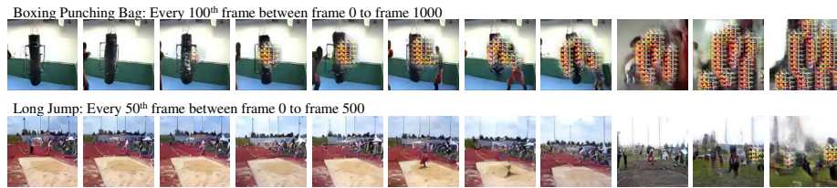
Fig. 19: Failure cases of class-conditional generation results of long videos on the UCF-101 dataset.
