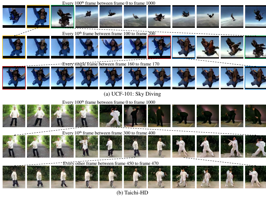
Fig. 18: Unconditional and class-conditional generation results of Sky Diving and Taichi-HD videos with 1,024 frames that contain smooth transitions.
