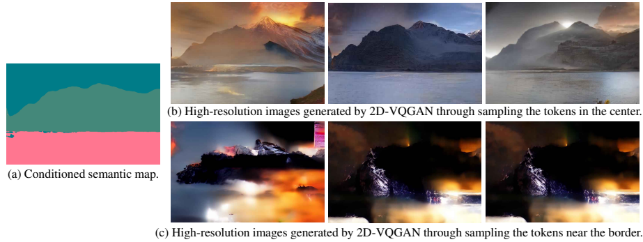
Fig. 12: 2D-VQGAN generates larger images by generating tokens in the center.
