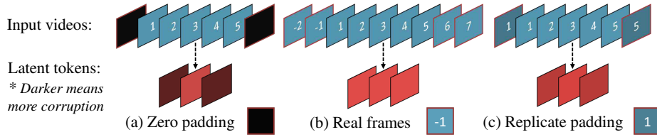
Fig. 4: Illustration of the temporal effects induced by paddings. Real frame padding makes the encoder temporally shift-equivariant 3 but introduces extra computations. Replicate padding makes decent approximation to the real frames while bringing no computational overhead.
