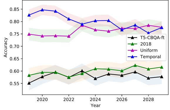
Figure 5: Accuracy over time of ordering pairs of queries from ( never , rare ) and ( rare , frequent ) sets based on the entropy assigned by the model.
