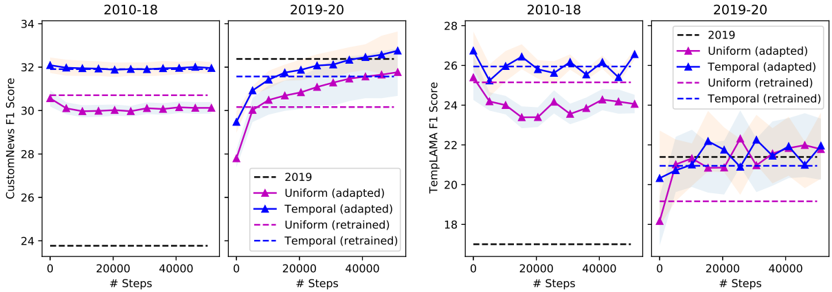
Figure 6: CUSTOMNEWS ( left ) and TEMPLAMA ( right ) F1 score as models are adapted to a mix of 50-50% data from 2010-18 and 2019. Dotted lines indicate models retrained from scratch on either 2019 alone or equal proportions of all data from 2010-19. The Temporal model does not degrade on the 2010-18 slice while adapted.
