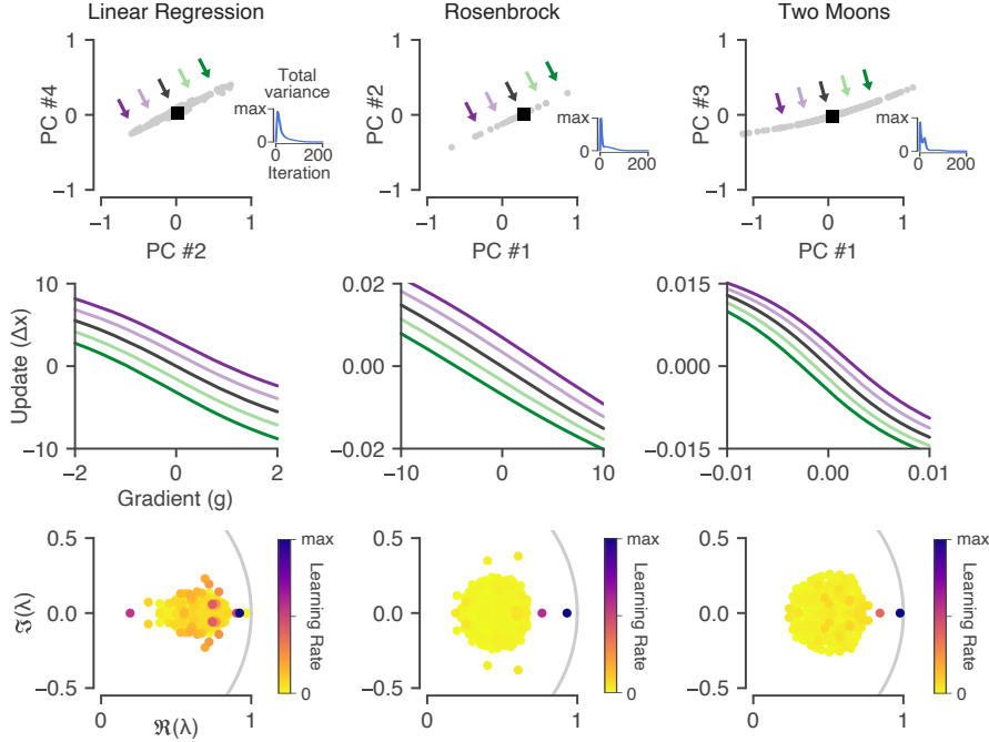
Figure 8: Momentum in learned optimizers. Each column shows the same phenomena, but for optimizers trained on different tasks. Top row : Projection of the optimizer state around a convergence point (black square). Inset : the total variance of the optimizer states over test problems goes to zero as the trajectories converge. Middle row : visualization of the update functions (§4.1) along the slow mode of the dynamics (colored lines correspond to arrows in (a)). Along this dimension, the effect on the system is to induce an offset in the update, just as in classical momentum (cf. Fig. 2c). Bottom row : Eigenvalues of the linearized optimizer dynamics at the convergence fixed point (black square in top row) plotted in the complex plane. The eigenvalue magnitudes are momentum timescales, and the color indicates the corresponding learning rate.
